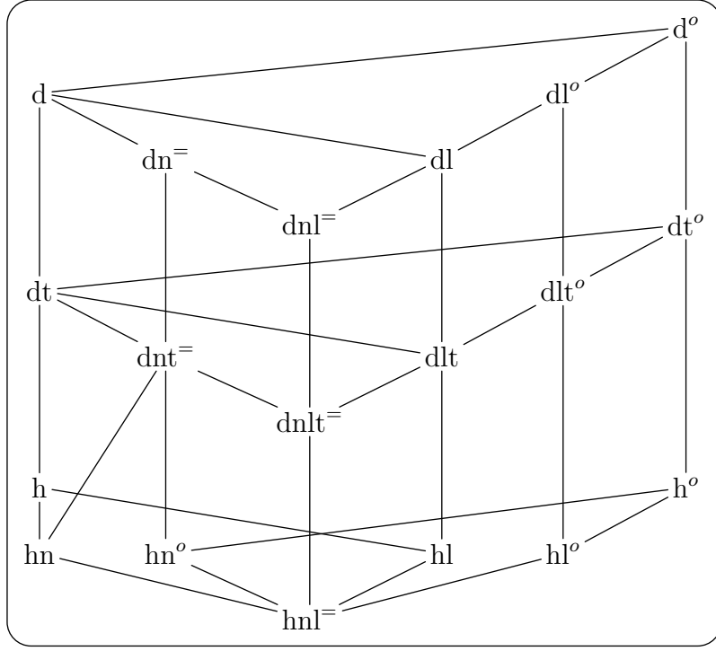
Fig. 4. HASSE diagram for periodic, commutative, and regular monoids, which are neither idempotent nor a group.
