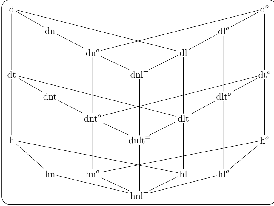
Fig. 3. HASSE diagram for periodic, commutative, and non-regular monoids.
