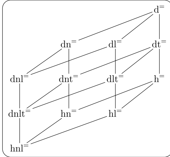
Fig. 1. HASSE diagram for the group \mathbb{Z}_2 .
