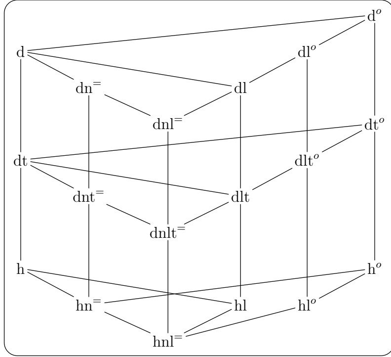
Fig. 5. HASSE diagram for commutative and idempotent monoids with at least three elements.
