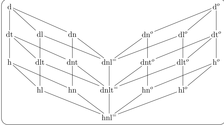
Fig. 2. HASSE diagram for non-periodic monoids.
