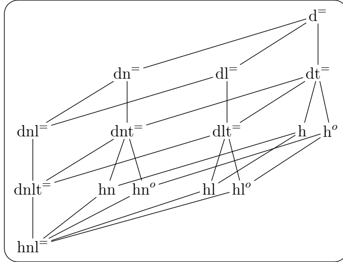
Fig. 6. HASSE diagram for periodic and commutative groups with an absorbing element \mathbf{0} and at least three elements.
