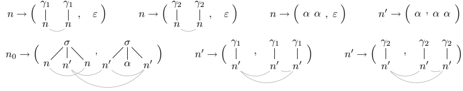
Fig. 1. Aligned example rules of the SFSG of Example 2.
