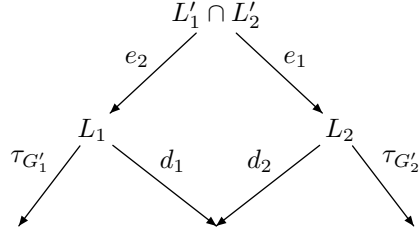
Fig. 3. Illustration of the approach used in the proof of Theorem 15.
