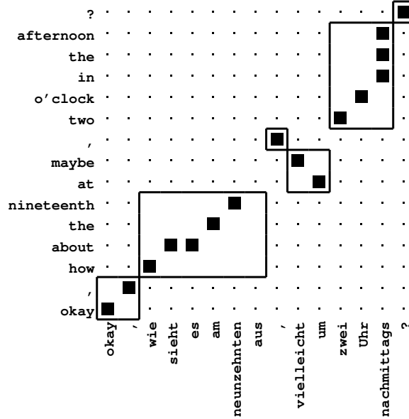
Figure 1.2: Example segmentation of German sentence and its English translation into alignment templates.
