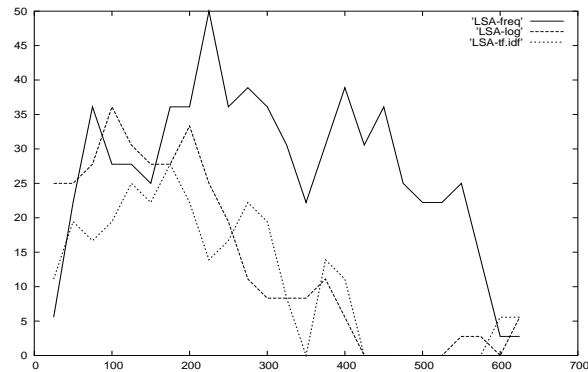
Figure 1: Precision for varying dimensions
