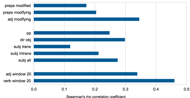
Figure 4: Syntax-based correlations.
