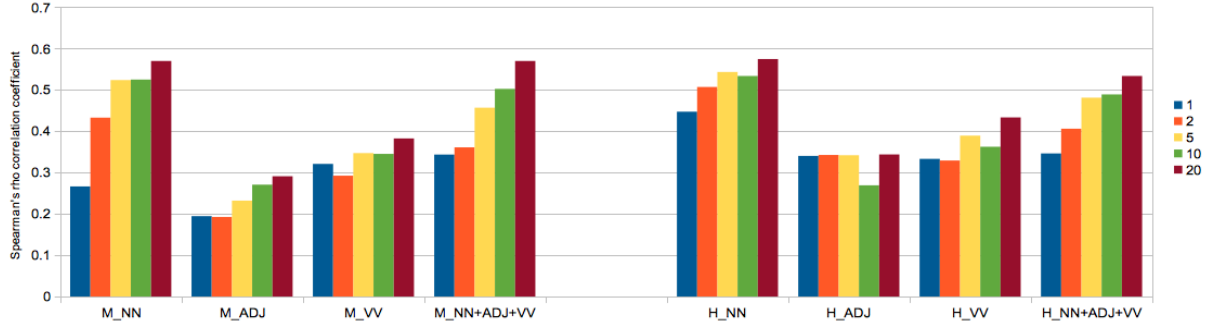
Figure 5: Window-based correlations (modifiers vs. heads).
