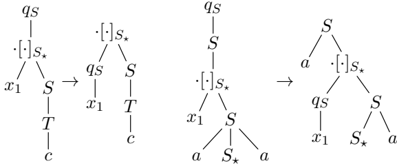
Figure 10: Two constructed XTT rules.
